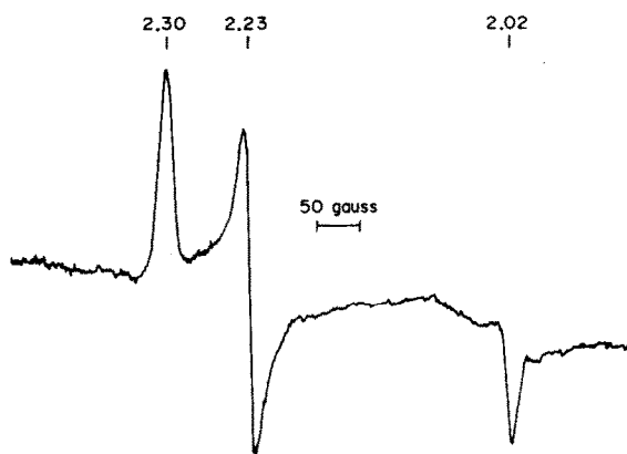
Fig. 2. EPR spectrum of oxidized membranes. Conditions: 9.24 GHz frequency, 20 G modulation amplitude, 10 mW power, 24 K, 4 \times 10^3 gain. Field positions calibrated by using a solution of reduced methyl viologen.
